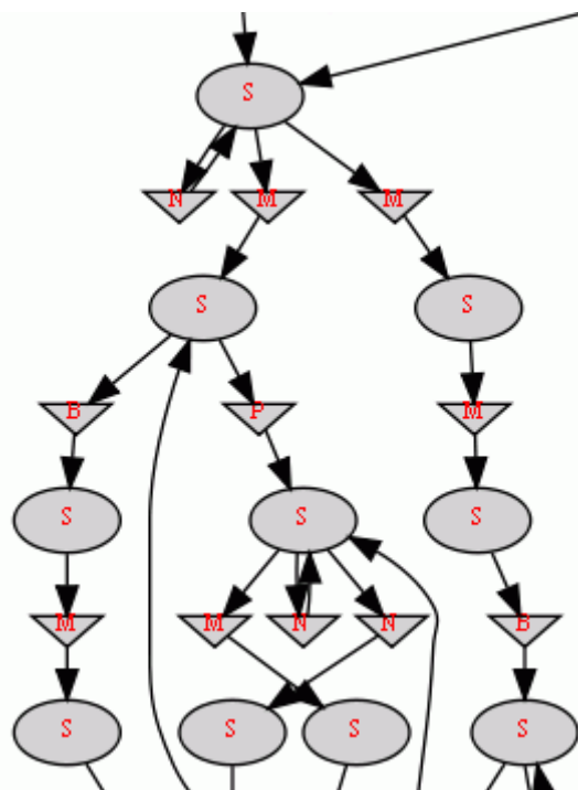
Figure 1. A fragment of acting graph (rendered with Graphviz package 13 ).
