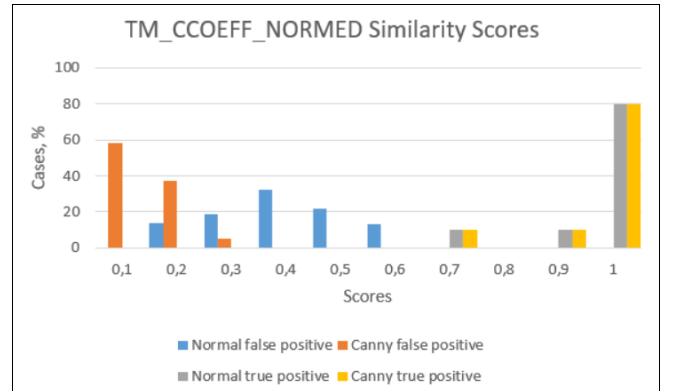
Figure 11. Struggling with false positive cases using Canny edge filtering.
